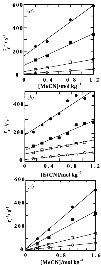
Fig. 2 Inverse of the mean lifetime of co-ordinated nitrile as a function of free nitrile concentration at different temperatures: (a) [Pd(MeCN) 4 ] 2+ 1 , ○ 297.4, □ 312.6, ■ 327.0, ● 337.0 K; (b) [Pd(EtCN) 4 ] 2+ 2 , ○ 301.5, □ 316.3, ■ 326.4, ● 336.4 K; (c) [Pd(MeCN) 4 ] 2+ 5 , ○ 300.1, □ 313.2, ■ 328.2, ● 338.2 K
