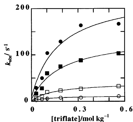
Fig. 3 Inverse of the mean lifetime of co-ordinated acetonitrile at [Pd(MeCN) 4 ] 2+ as a function of triflate concentration at different temperatures. No free acetonitrile was added. ○ 296.8, □ 311.3, ■ 326.3, ● 337.2 K
